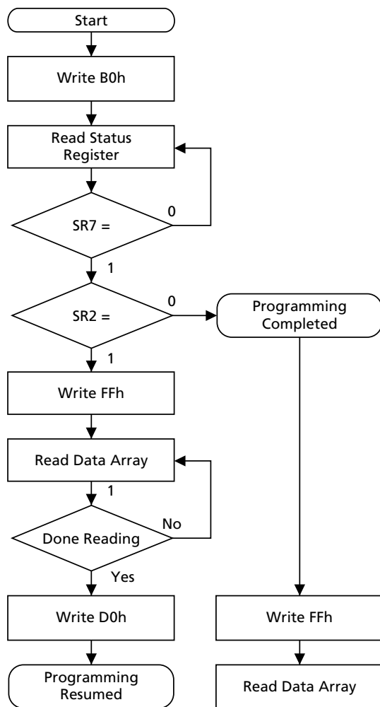
Figure 11: PROGRAM SUSPEND/RESUME
