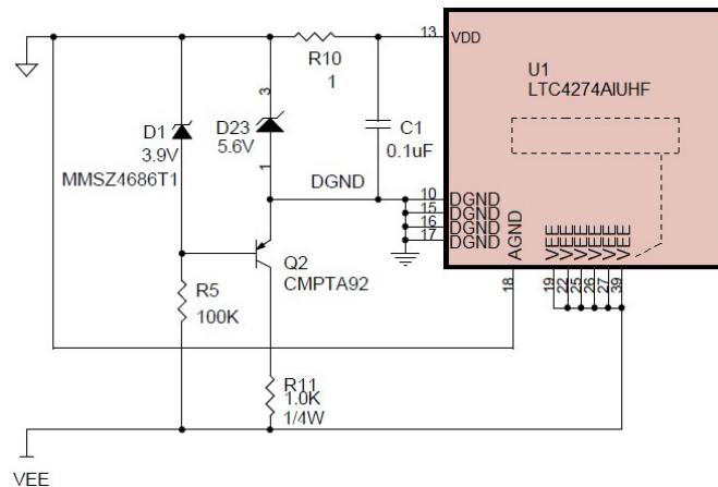
Figure 4. DC1814A LDO Circuit for the LTC4274A Digital Supply
