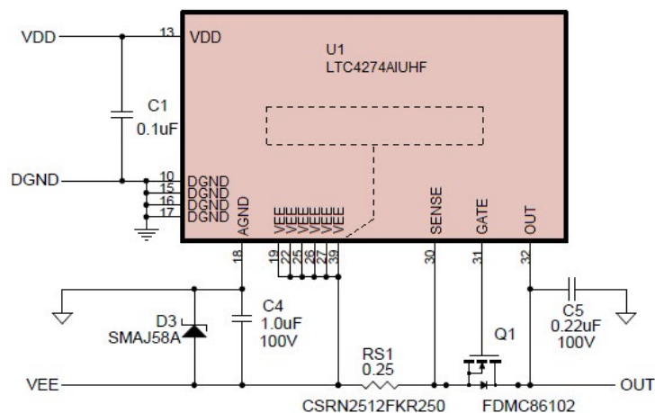
Figure 2. LTC4274A Key Application Components for Board Placement
