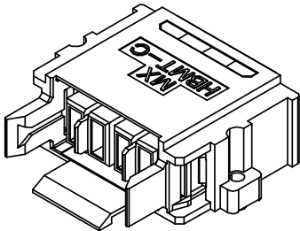
ISOMETRIC VIEW RIVET MOUNTING
