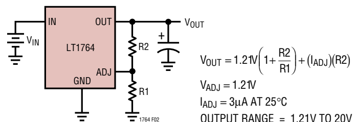
Figure 2. Adjustable Operation
