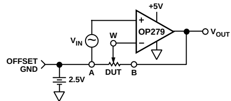
Figure 31. Noninverting Programmable Gain Test Circuit
