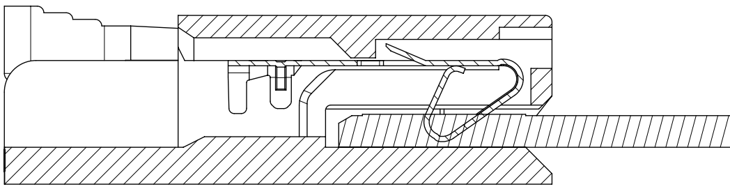
TERMINAL-HOUSING AND PCB AS ASSEMBLED
