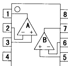
NJM2147D NJM2147M
