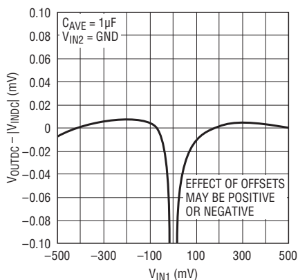
DC Linearity
