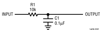
Figure 2. Lowpass Filter for PWM Averaging
