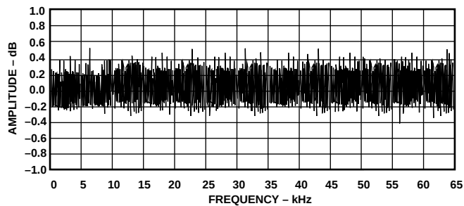
Figure 19. DNL Plot at V_{REF} = 10 V, T_A = +25^\circ\text{C} , f_S = 100 kSPS
