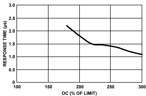
FIGURE 14. RESPONSE TIME vs I_O \cdot R_{SNS}
