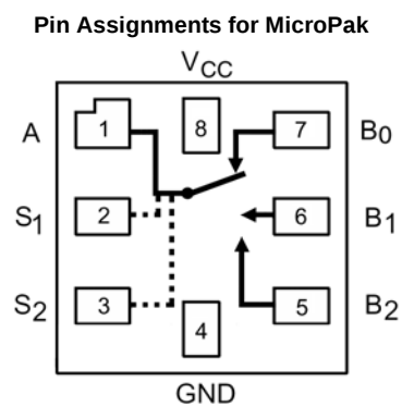
(Top Through View)
