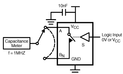
FIGURE 7. Channel Off Capacitance
