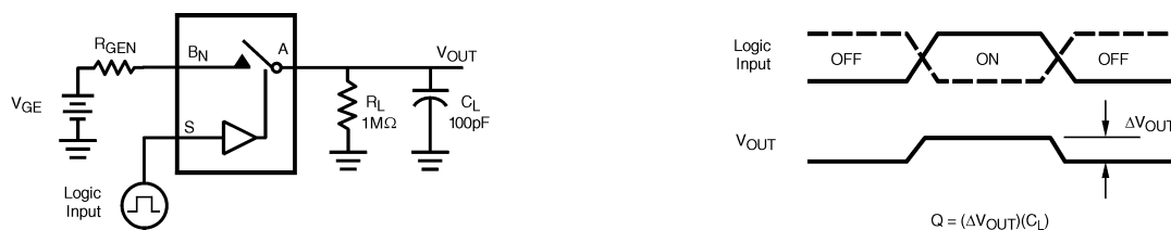
FIGURE 4. Charge Injection Test
