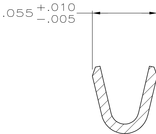
SECTION Y-Y SCALE 20:1
