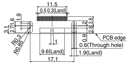
◆ Recommended PCB mounting pattern
