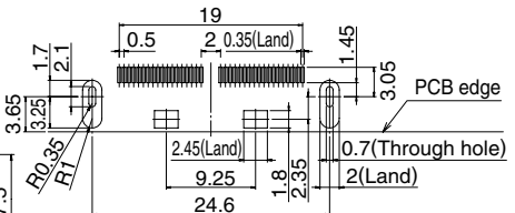
◆ Recommended PCB mounting pattern
