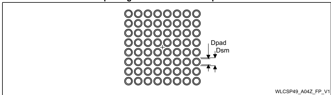
Figure 56. WLCSP64 - 64-ball, 3.141 x 3.127 mm, 0.35 mm pitch wafer level chip scale package recommended footprint
