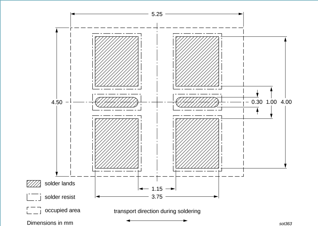
Fig 16. Wave soldering footprint BAV756S and BAW56S (SOT363/SC-88)
