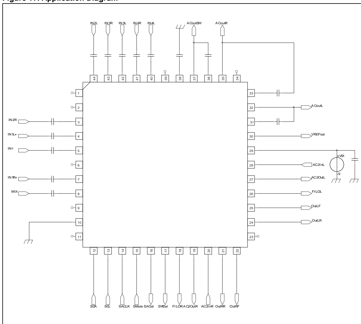
Figure 17. Application Diagram
