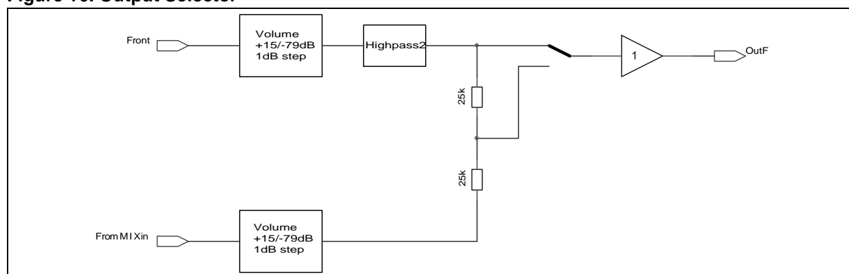
Figure 16. Output Selector
