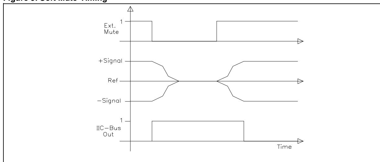
Figure 5. Soft Mute-Timing
