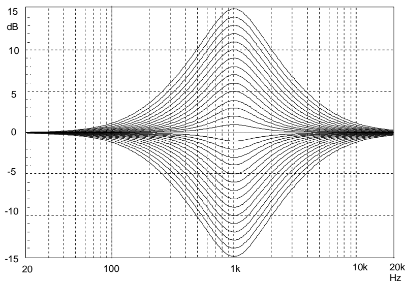
Figure 7. Equalizer filter control @ f_{\text{Center}} = 1\text{kHz} , Q = 1.0
