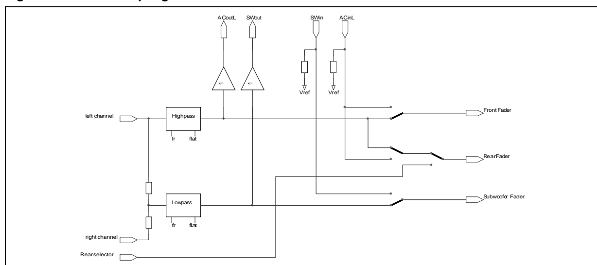
Figure 15. AC/DC-coupling
