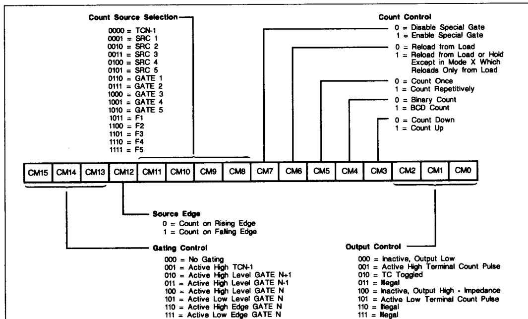
Figure 16. Counter Mode Register Bit Assignments
