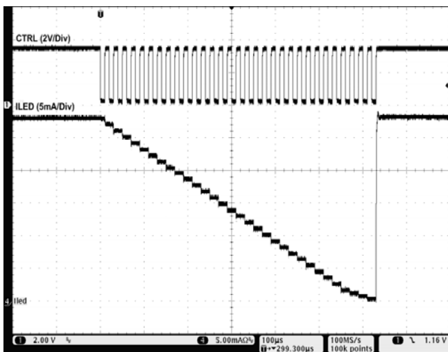
Figure 16. Dimming Operation
