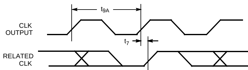
Figure 4. CLK Outputs Jitter and Skew
