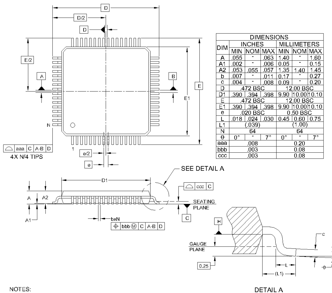
Figure 18 LQFP Package
