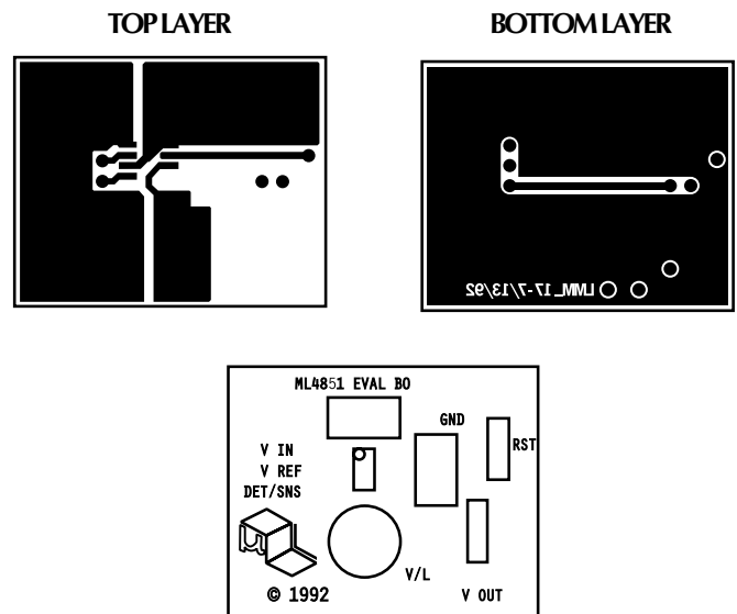
Figure 6. Sample PC Board Layout
