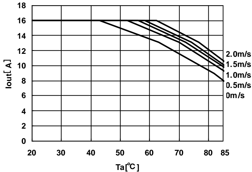
Thermal Derating (MPDTY311S)
