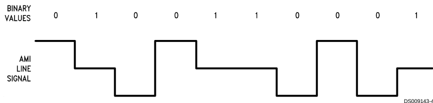
FIGURE 1. Inverted AMI Line-Coding Rule
