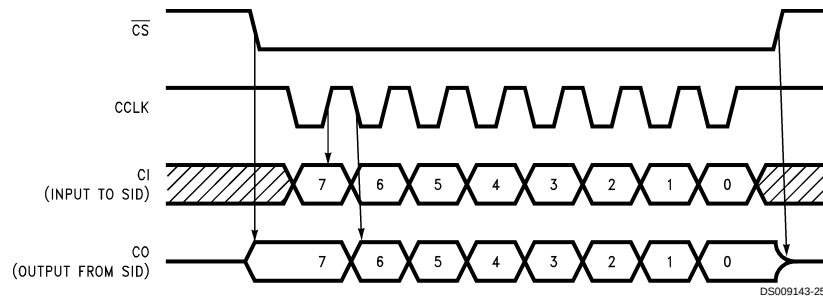
FIGURE 8. TP3420A Alternate MICROWIRE Clock Format
