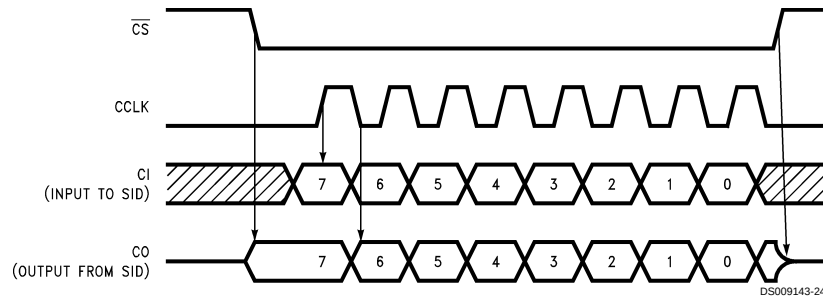
FIGURE 7. TP3420A Normal MICROWIRE Clock Format
