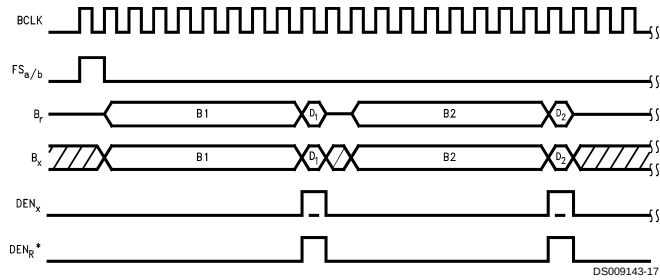
FIGURE 4. Digital System Interface Formats in TEM mode (DSI Master)
