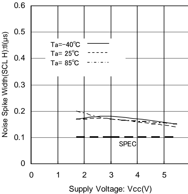
Figure 27. Noise Spike Width vs Supply Voltage (SCL H)
