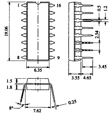
16-Lead DIL Plastic Package (16-DIP)
