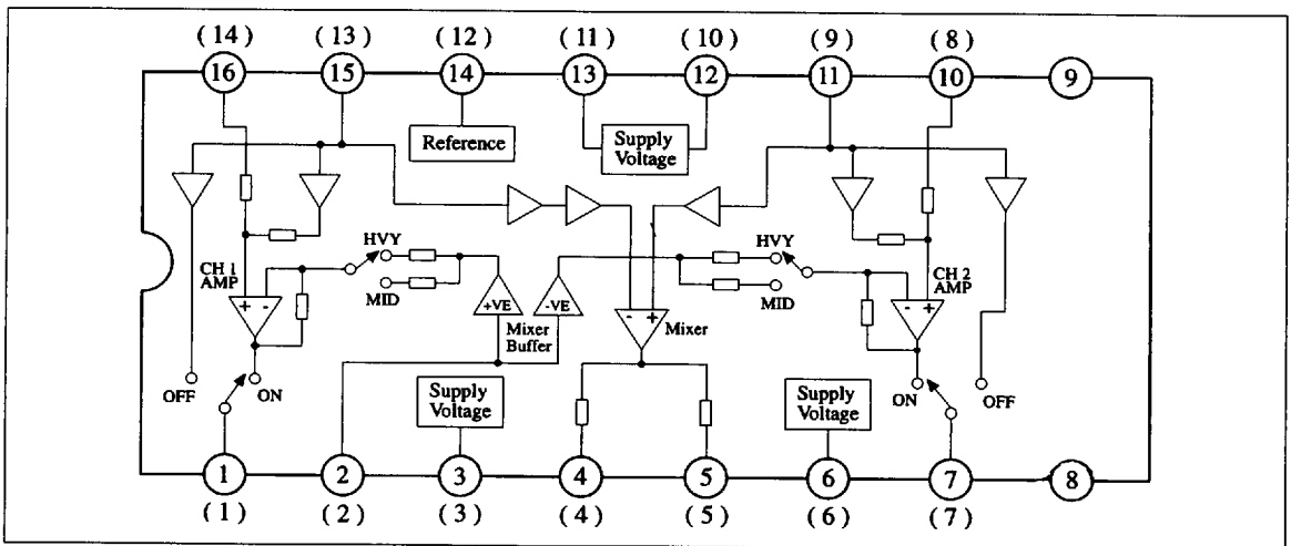
14-Lead PANAFLAT Plastic Package (SO-14D)
