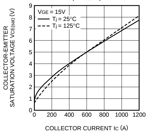
COLLECTOR-EMITTER SATURATION VOLTAGE CHARACTERISTICS (TYPICAL)
