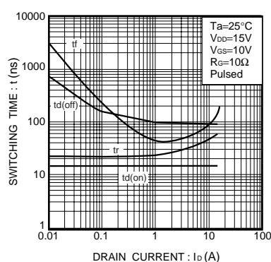
Fig.2 Switching Characteristics
