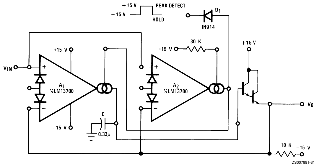
FIGURE 24. Peak Detector and Hold Circuit
