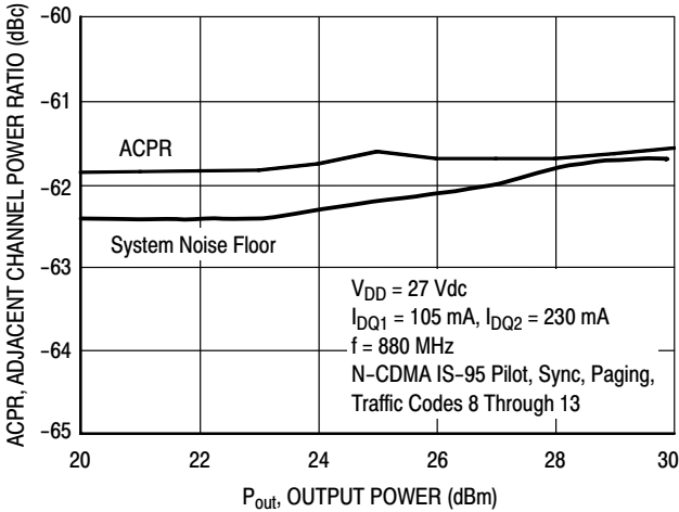
Figure 15. Single-Carrier N-CDMA ACPR versus Output Power
