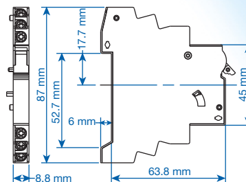
Dimensions HxxUM.
