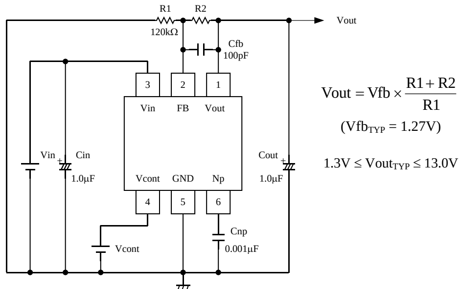
Figure 8. External Circuit
