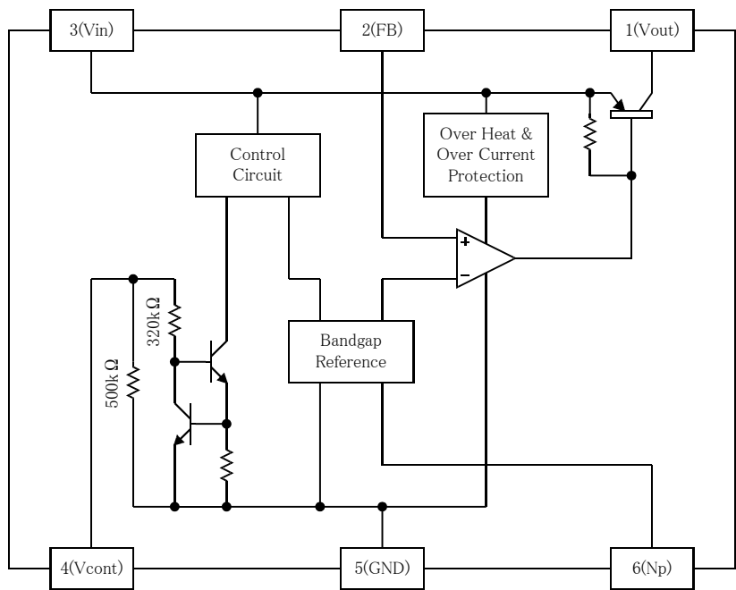
Figure 1. Block Diagram
