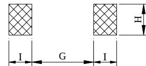
PCB PATTERN
