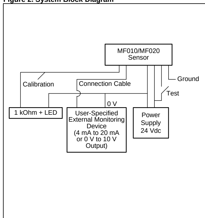
Figure 2. System Block Diagram
