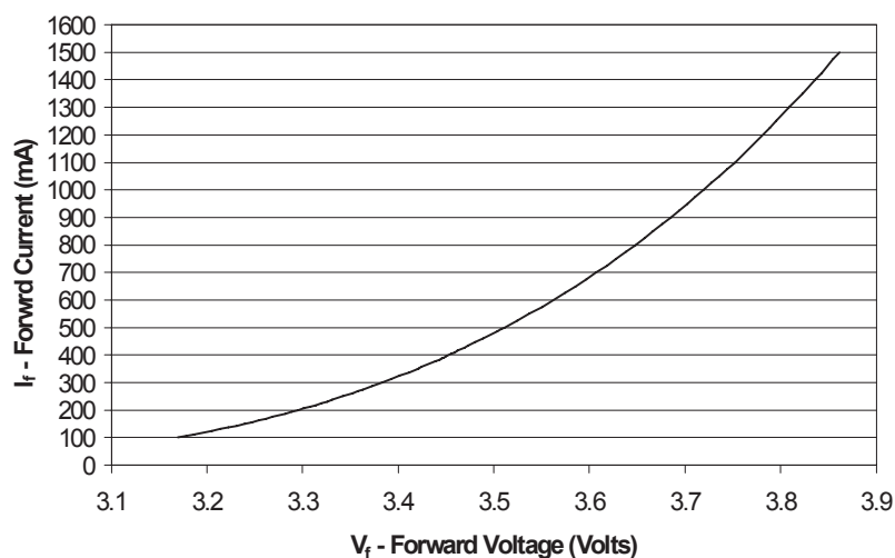
Figure 9. Forward current vs. forward voltage for white, green, cyan, blue and royal blue.
