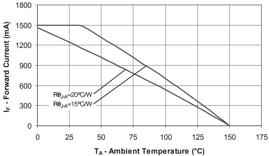
Figure 21: Maximum forward current vs. ambient temperature, based on T JMAX = 150°C.
