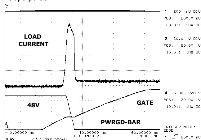
FIGURE 26. INRUSH CURRENT
