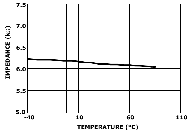
FIGURE 21. PWRGD (ISL6150) IMPEDANCE ( k\Omega )
