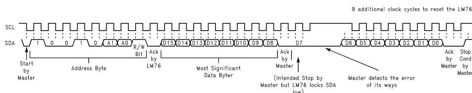
Figure 7. Inadvertent 8-Bit Read from 16-Bit Register where D7 is Zero (“0”)
