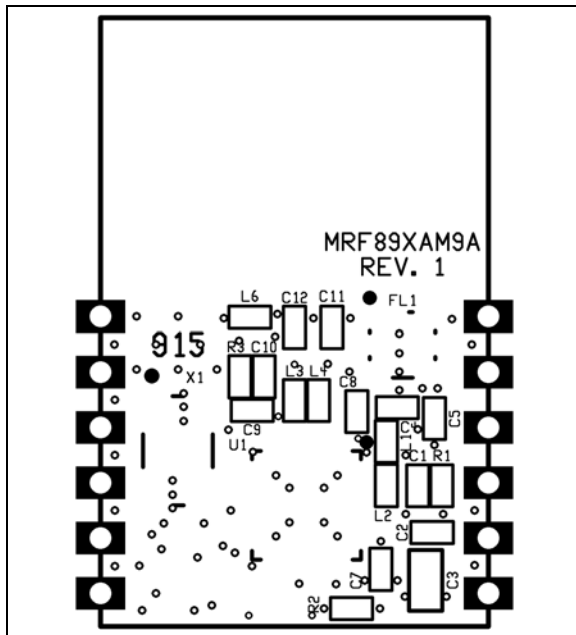
FIGURE 2-4: TOP COPPER
