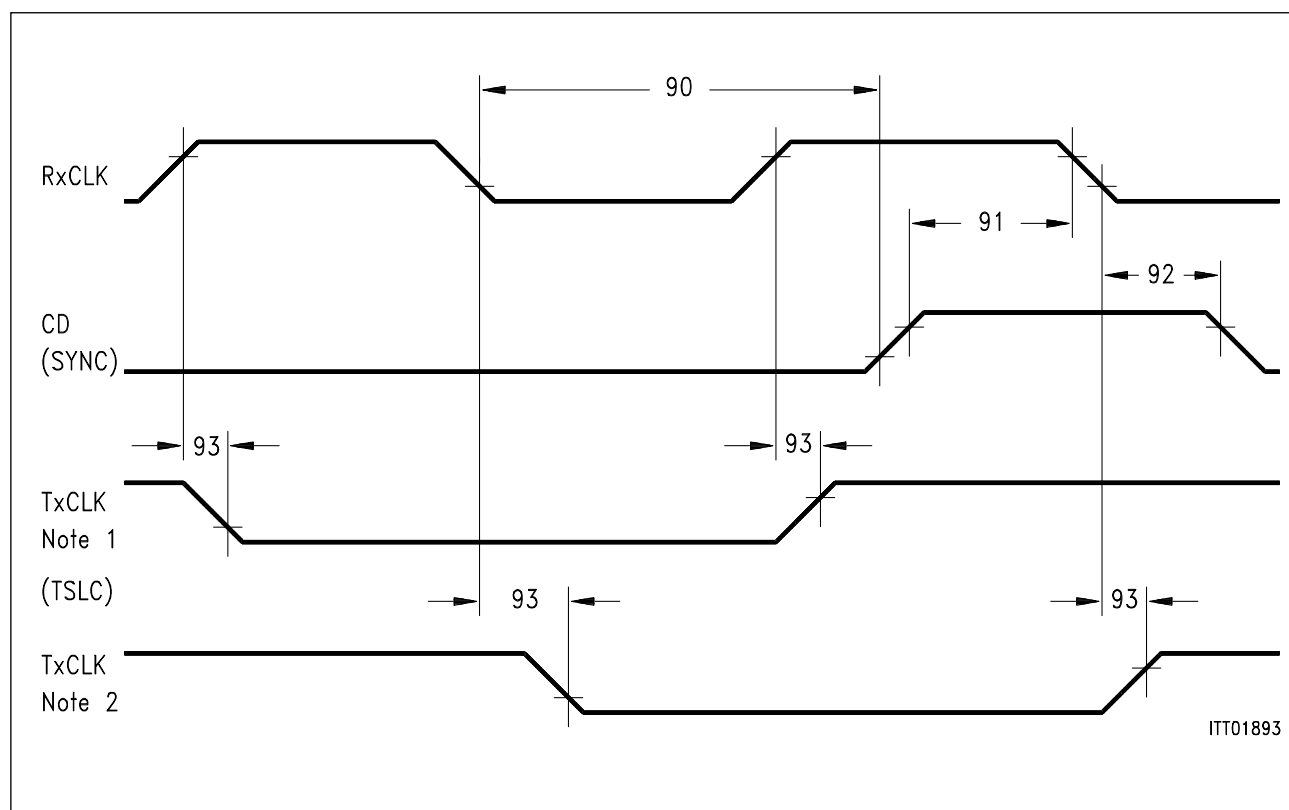
Figure 70 Synchronization Timing
