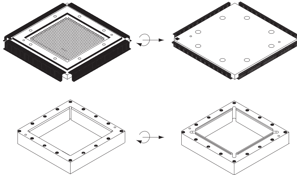
Figure 12 • Upside Down View of CQ352 to FG896 Ceramic Adapter and Socket Housing
