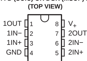
TLV342 . . . D (SOIC) OR DGK (MSOP) PACKAGE
