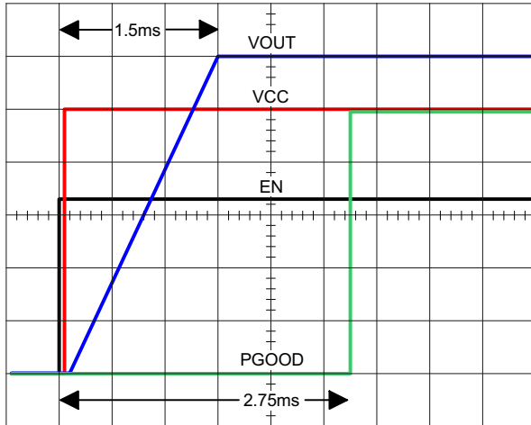
FIGURE 4. SOFT-START SEQUENCE
