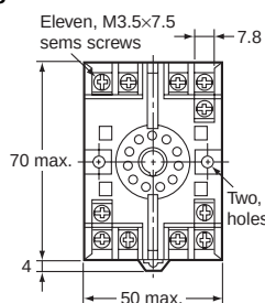
P2CF-11 Front Connecting Socket
