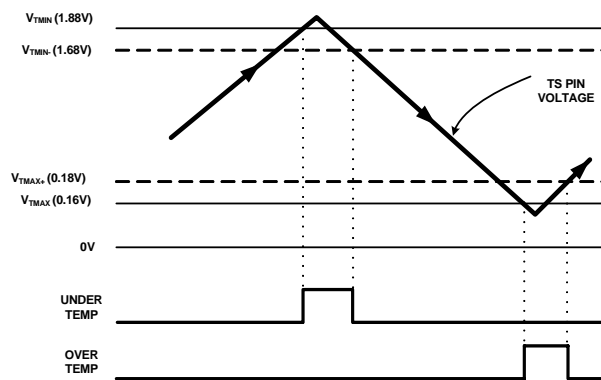
FIGURE 1. THRESHOLD VOLTAGES FOR 0°C to +50°C WINDOW
