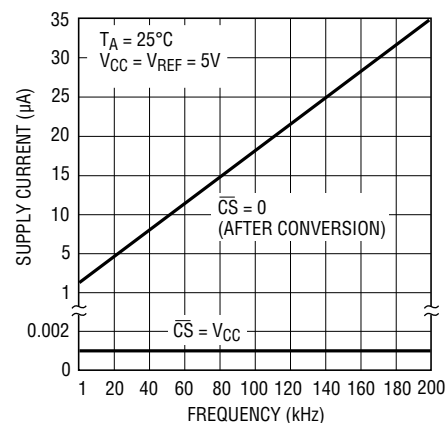
Shutdown Supply Current vs Clock Rate with \overline{\text{CS}} High and \overline{\text{CS}} Low
