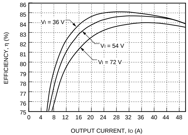
Figure 5. Typical FW250A1 Efficiency vs. Output Current at Room Temperature
