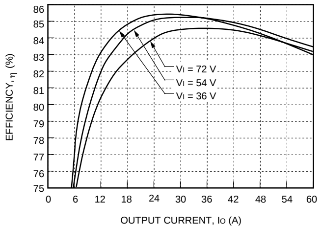
Figure 6. Typical FW300A1 Efficiency vs. Output Current at Room Temperature
