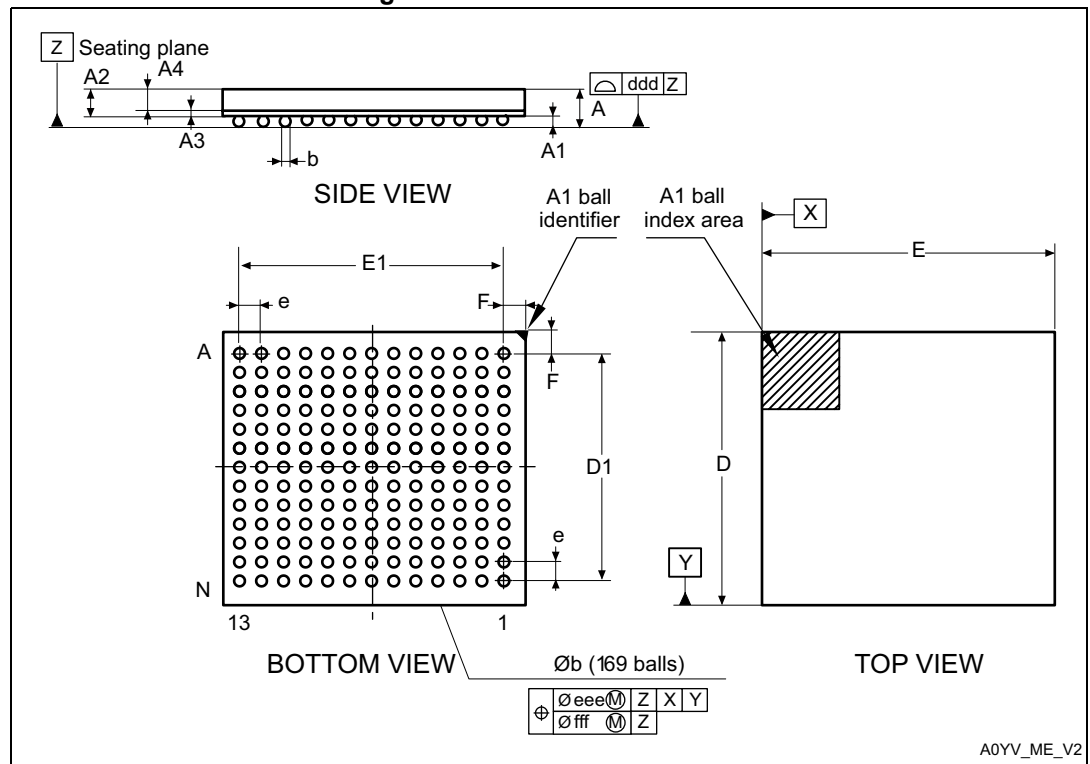
Figure 84. UFBGA169 - Outline
