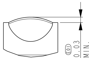
DETAIL A SCALE 50:1
