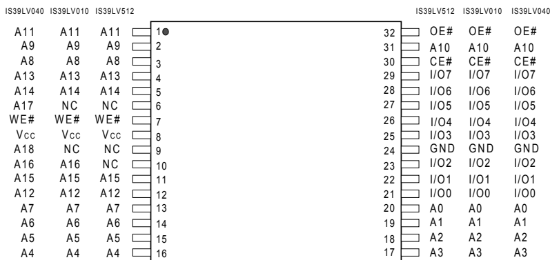
32-Pin VSOP
