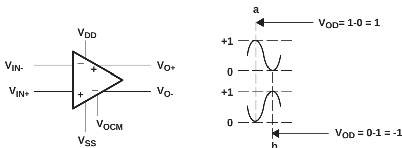
Figure 27. Fully Differential Amplifier With Two 1- V_{PP} Signals
